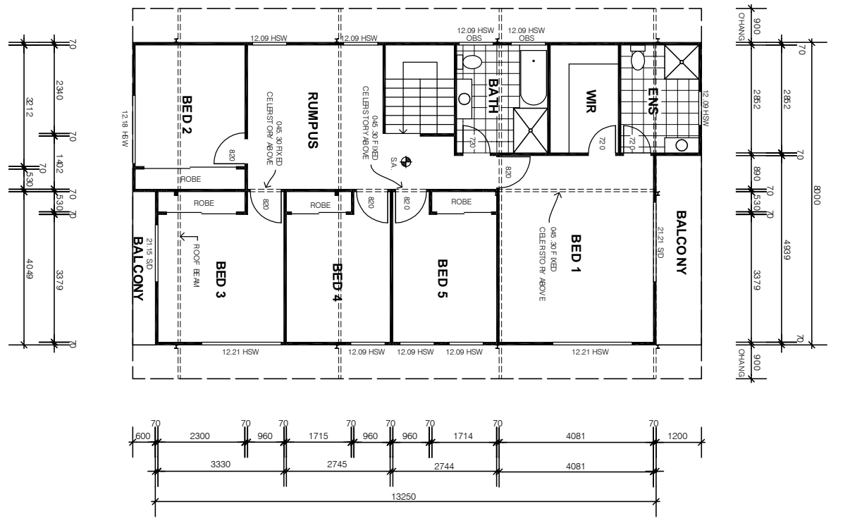
SECOND FLOOR
