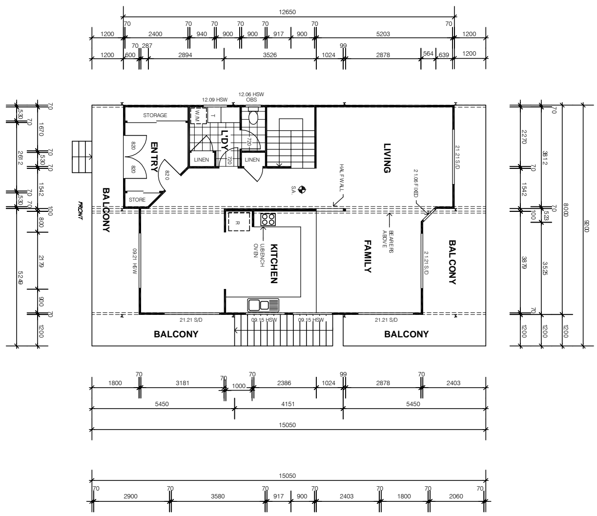
FIRST FLOOR
