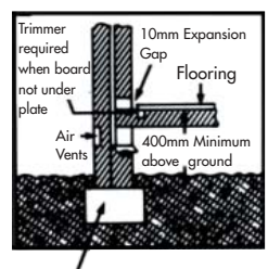
Fitted floor
