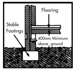
Platform construction
