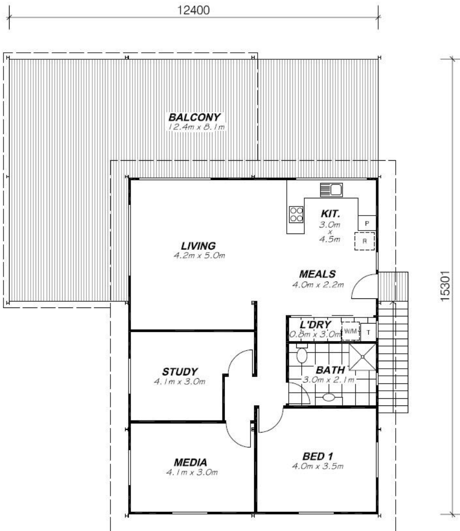
FLOOR PLAN
